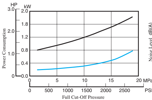
Power Consumption at Full Cut-Off Pressure
