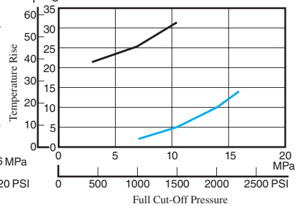
Characteristics of Oil Temperature Increase in the Reservoir
